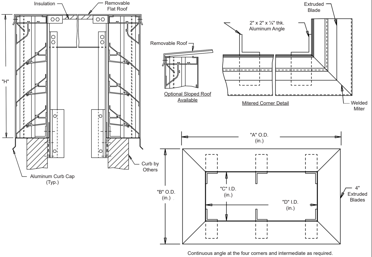
Continuous angle at the four corners and intermediate as required.
